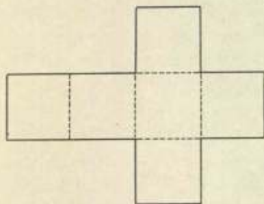
CUBE.
